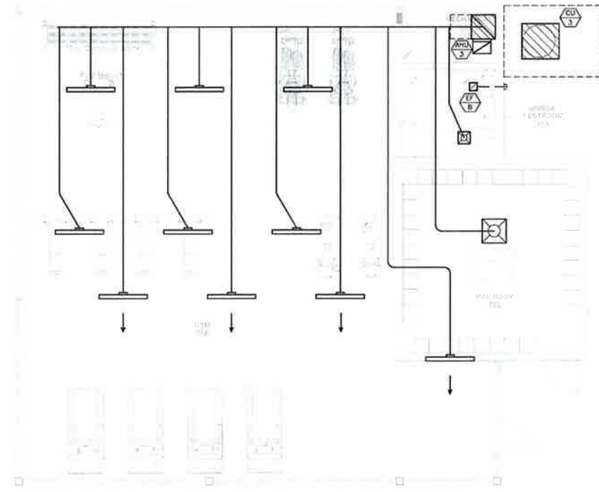
1 GYM - MECHANICAL SCALE: 1/4"=1'-0"
