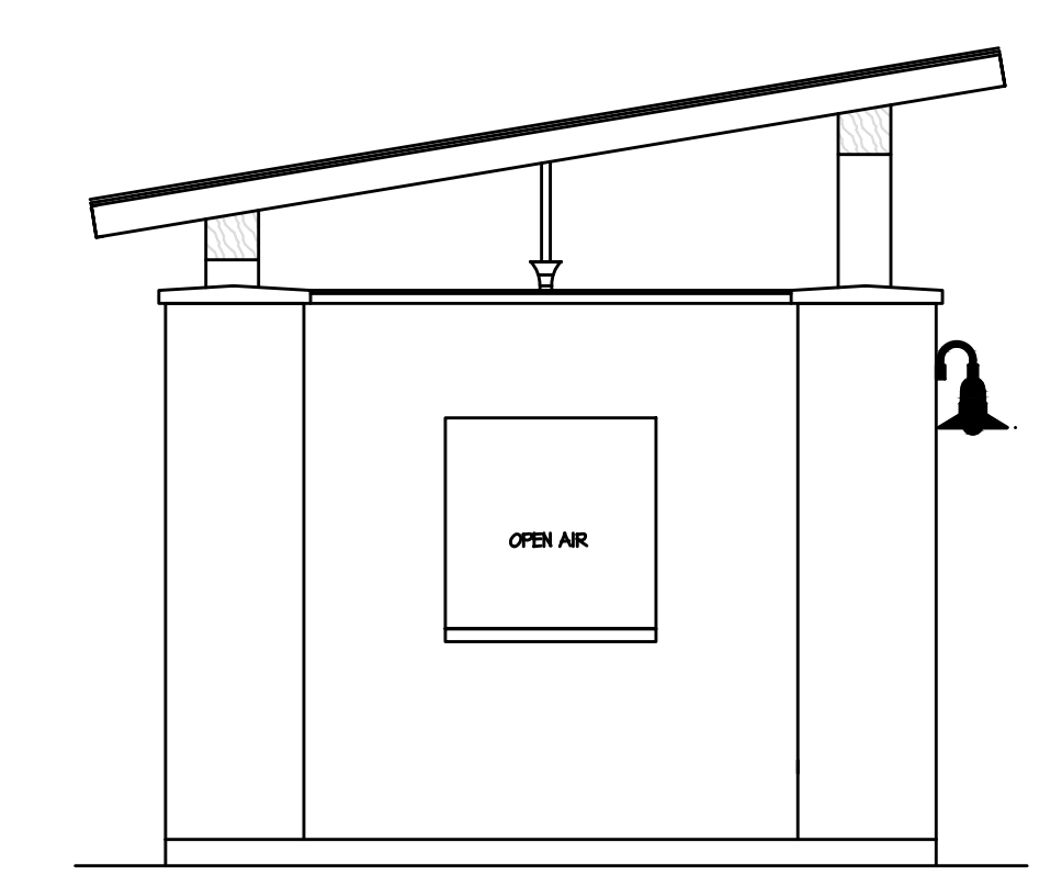
LEFT SIDE VIEW LIGHTING N.T.S.
