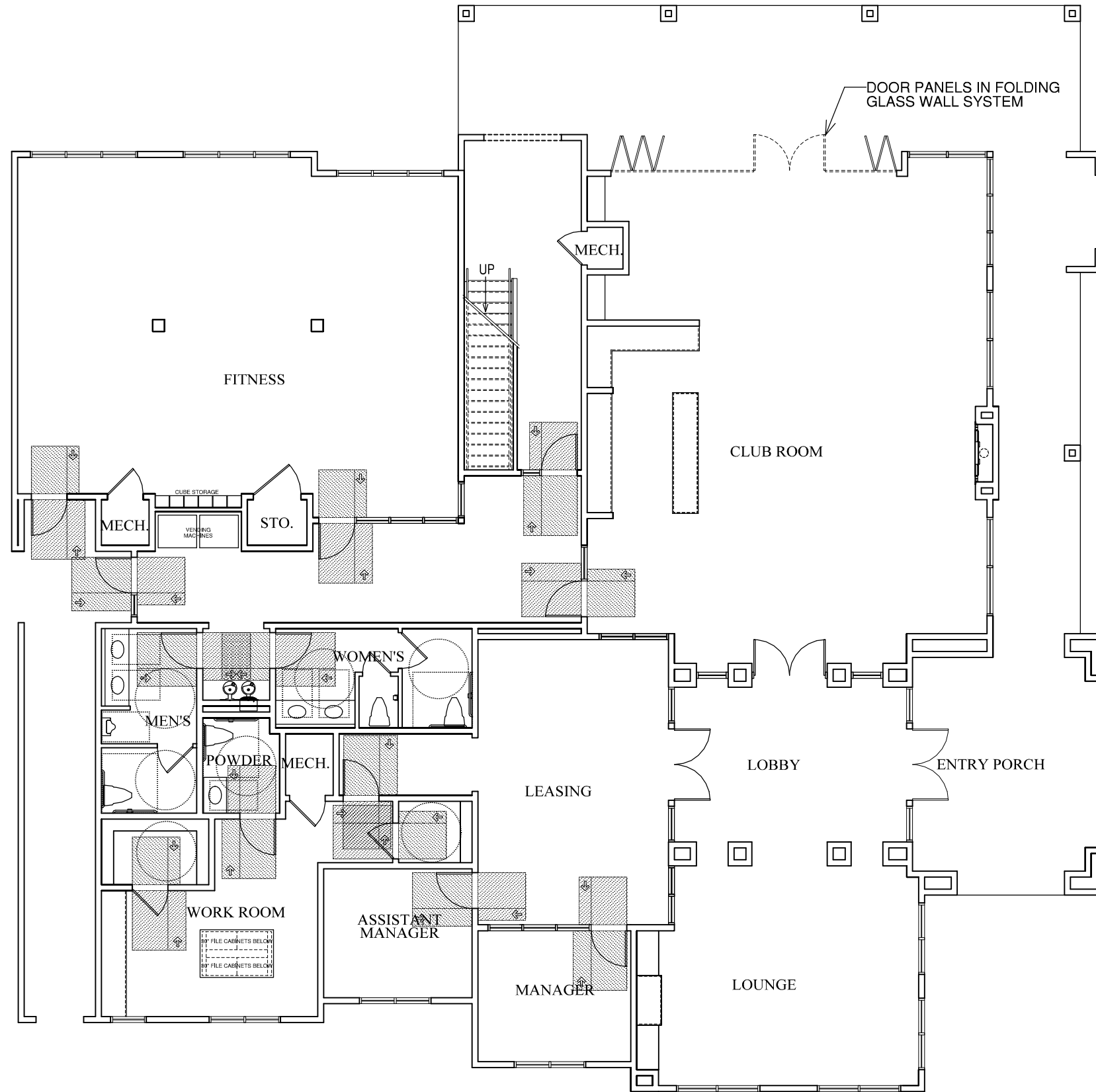
CLUB PLAN SCALE 3/32"=1'-0"
