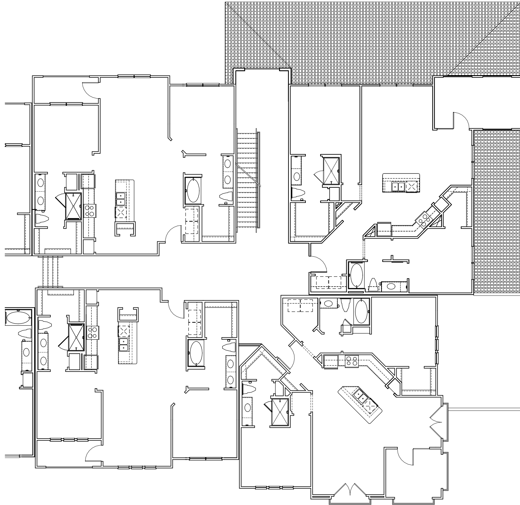
UNITS ABOVE CLUB SCALE 3/32"=1'-0"
