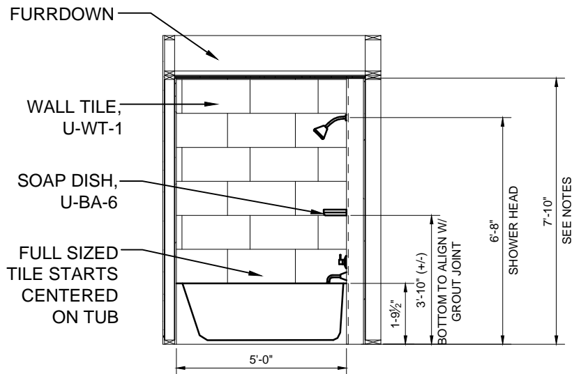
1 TYP. TUB/SHOWER TILE PATTERN SCALE 1/4"=1'-0"
