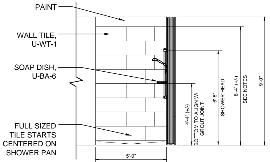
1 TYP. SHOWER TILE PATTERN SCALE 1/4"=1'-0"
